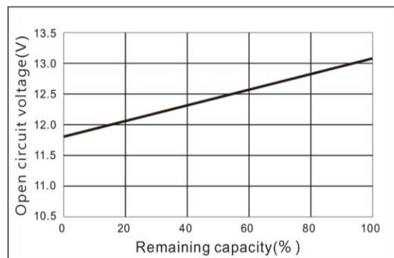
Curves of open circuit voltage vs. capacity
