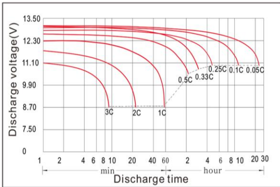
Discharge characteristic
