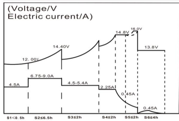
Charging characteristic
